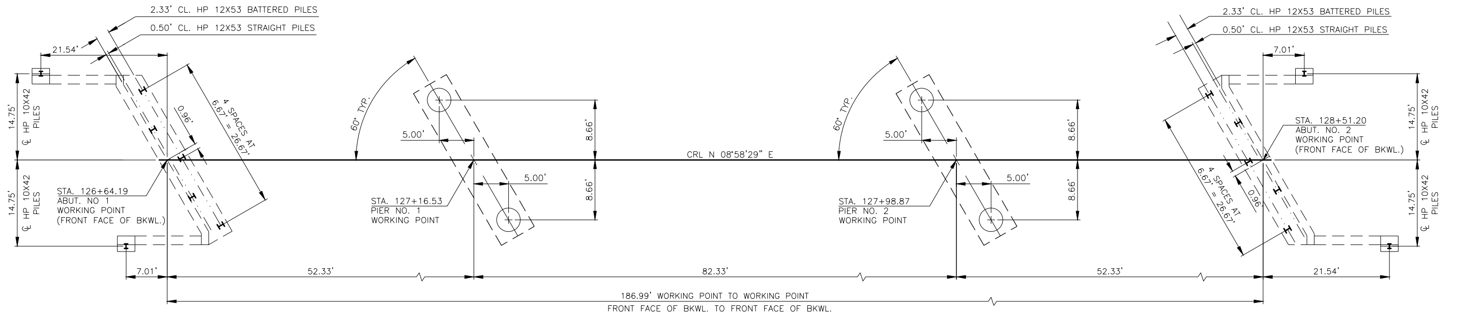
STAKING DIAGRAM BRIDGE "A"
